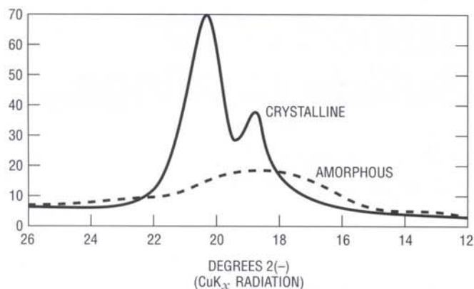
Figure 1 — X-ray diffraction patterns of PPS
