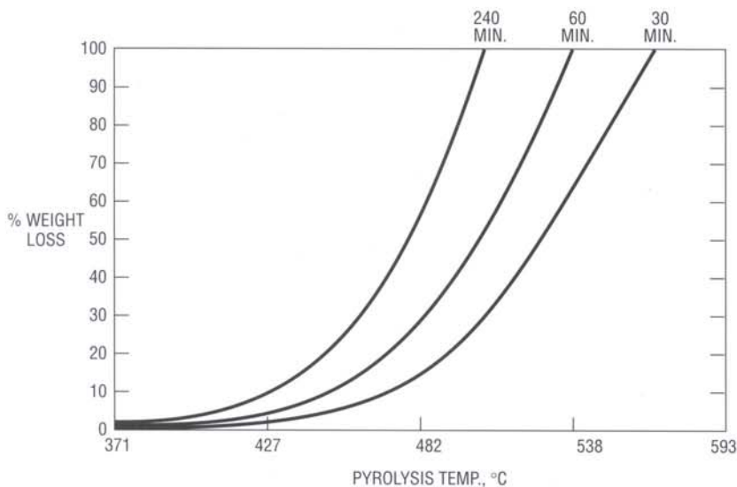
Figure 2 — Weight loss of PPS in air
