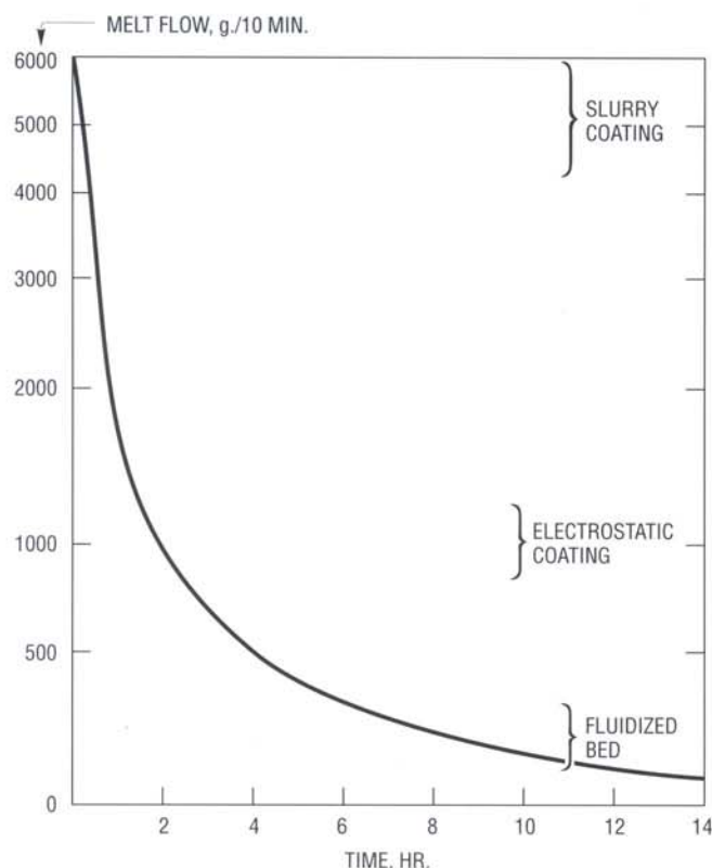
Figure 3 — Preparation of PPS coating resins by precuring at 232°C
